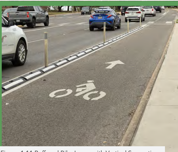
Figure 1.11 Buffered Bike Lanes with Vertical Separation
